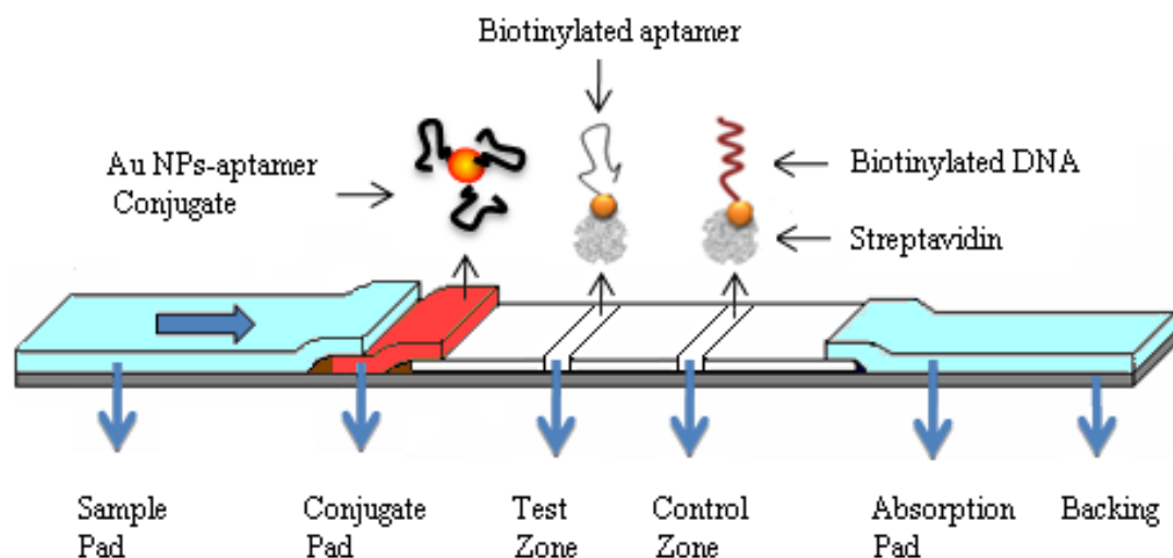
Fig. S1. Schematic diagram of aptamer-nanoparticle strip biosensor based on aptamer-functionalized gold nanoparticle probes and lateral flow test strip for detection of cancer cells.
