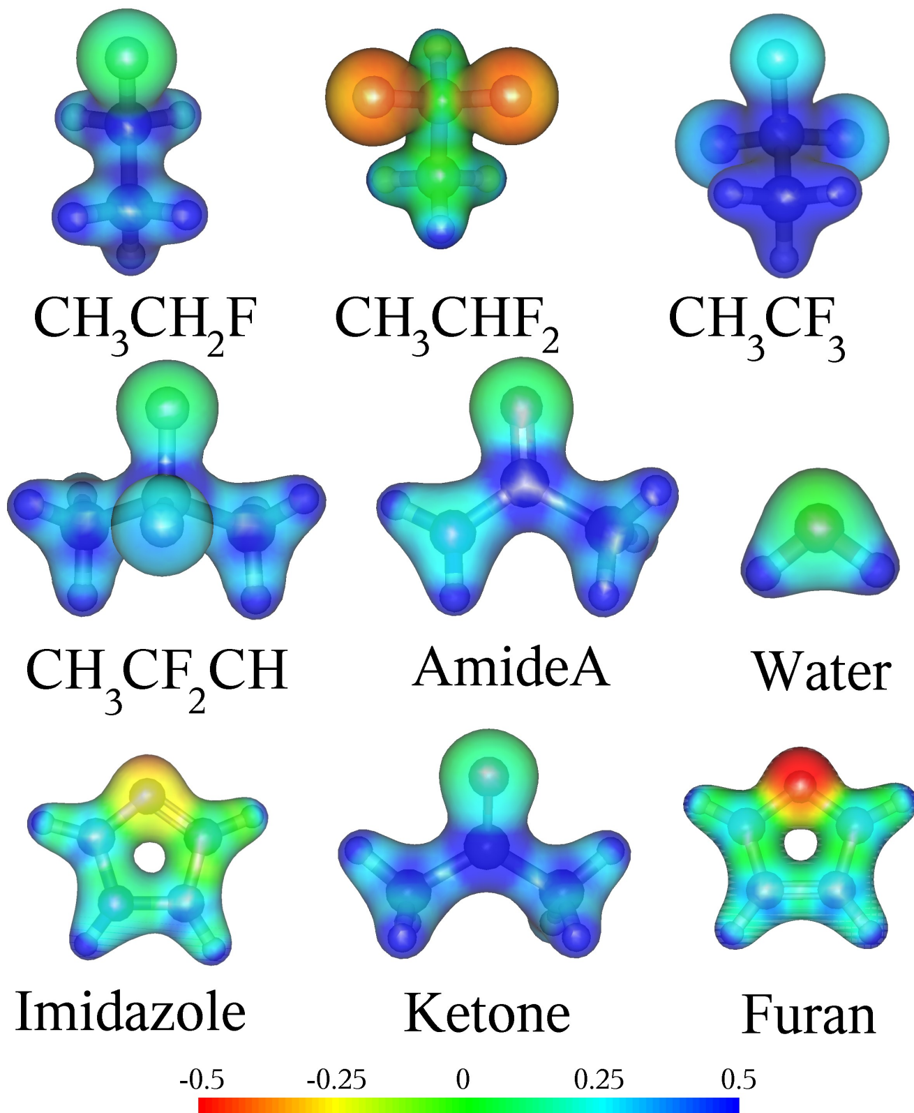
Supplementary File 7. Electrostatic potential of H-bond acceptors. All isovalues are represented within the same scale of potential. B3LYP (6-311G**++) optimization.
