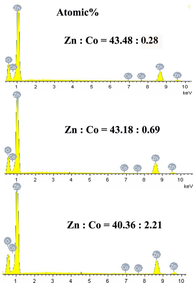
Figure S1. SEM EDX spectra of three as-prepared Co-doped ZnO samples with different levels of doping.
