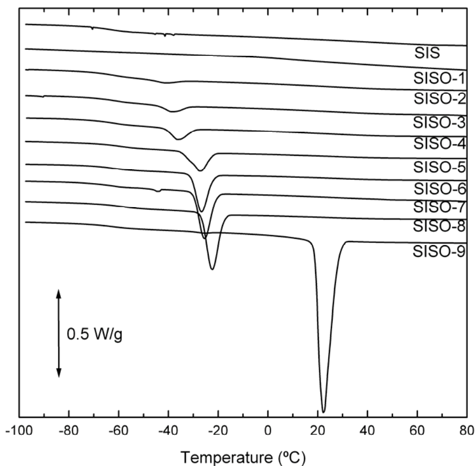
Figure S.1 Cooling DSC scans (10 °C/min) of SIS triblock and SISO tetrablocks after heating to 150 °C.
