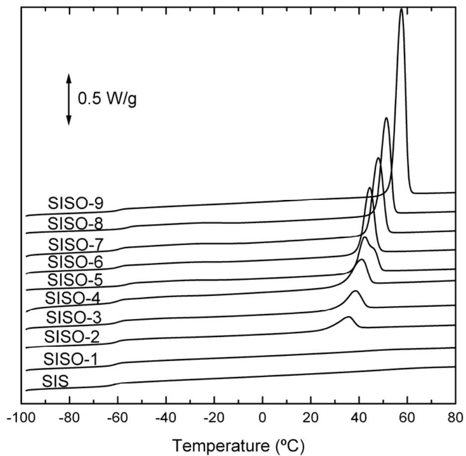
Figure S.2 Heating DSC scans (10 °C/min) of SIS triblock and SISO tetrablocks after cooling to -100\text{ }^{\circ}\text{C} (data shown in Figure S.1).
