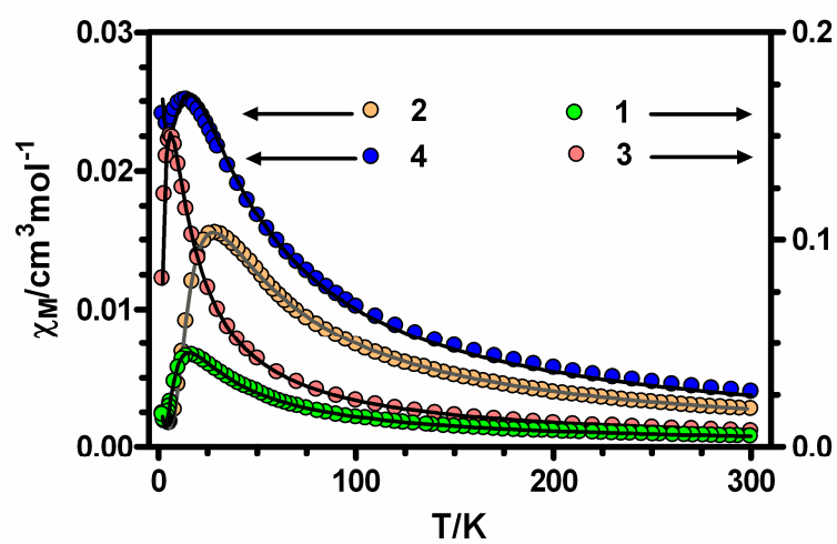
Figure 6. Temperature dependence of \chi_M for compounds 1-4. As indicated by the arrows, 1 and 3 are represented on right axis whereas 2 and 4 are represented on the left axis.
