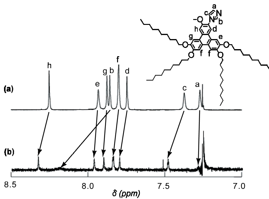
Fig. S3 ^1\text{H} NMR spectra of 2 (a) and the mixture of 2 and \text{AgNO}_3 (b) in \text{CDCl}_3
