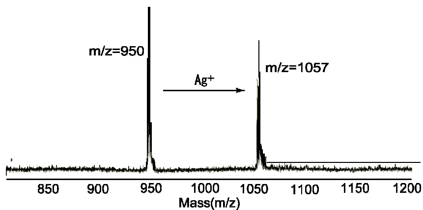
Fig. S2 MALDI-TOF mass spectrum of 2 with \text{AgNO}_3
