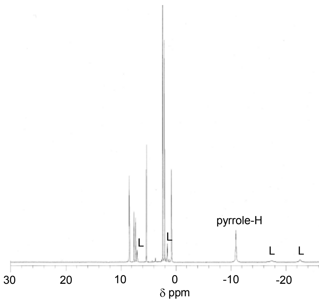
Figure S1. ^1\text{H} NMR spectrum of [\text{Fe}(\text{THFPrP})(3\text{-MePy})_2]^+ taken in \text{CD}_2\text{Cl}_2 at 298 K.
