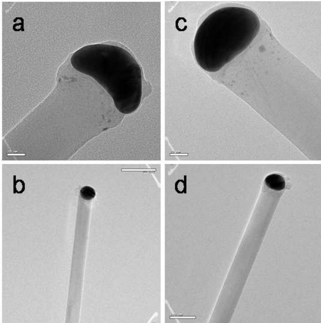
Figure S1: TEM images of the as-grown (a, b) and annealed (c, d) nanowires. Scale bars are: 20nm, 200nm, 20nm and 100nm for (a) , (b) , (c) , and (d) , respectively.
