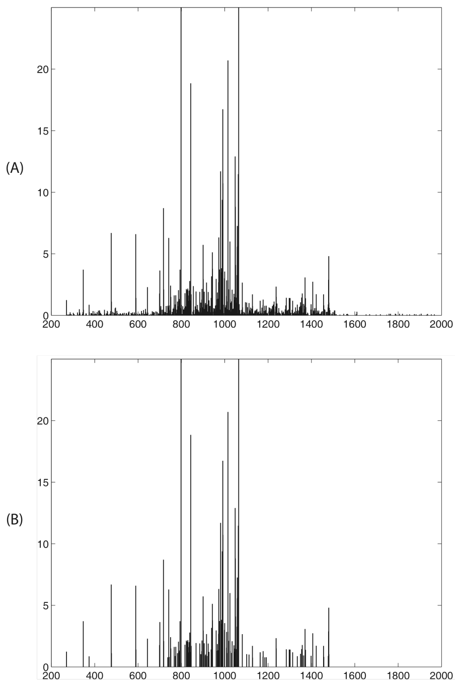
Supplementary Figure S3: Denoising of an MS/MS spectrum. Comparison of the raw experimental spectrum (A) and denoised spectrum (B). The major signal peaks remain intact after ~80% of the peaks are removed.
