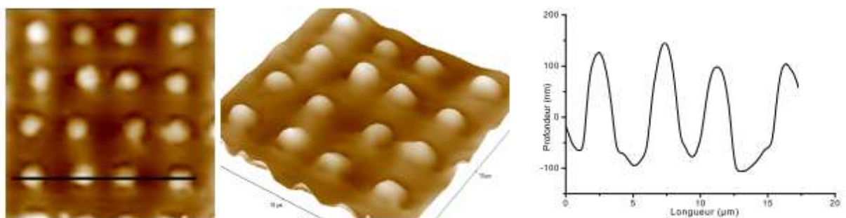
SI-5. AFM image and profile of the fourth replica obtained without cleaning from master mold A.
