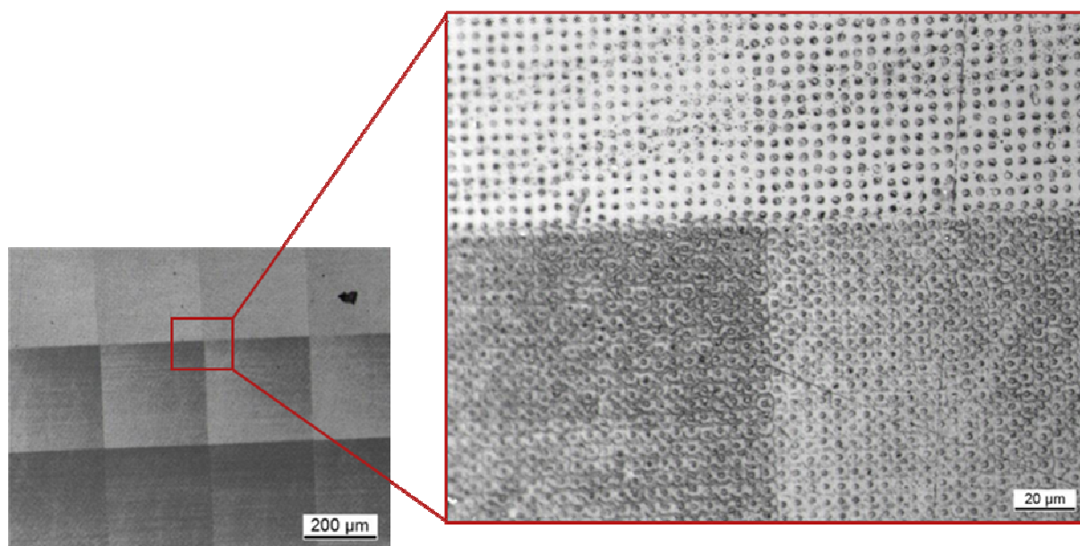
SI-1. Image by ESEM of the junction between four matrices.
