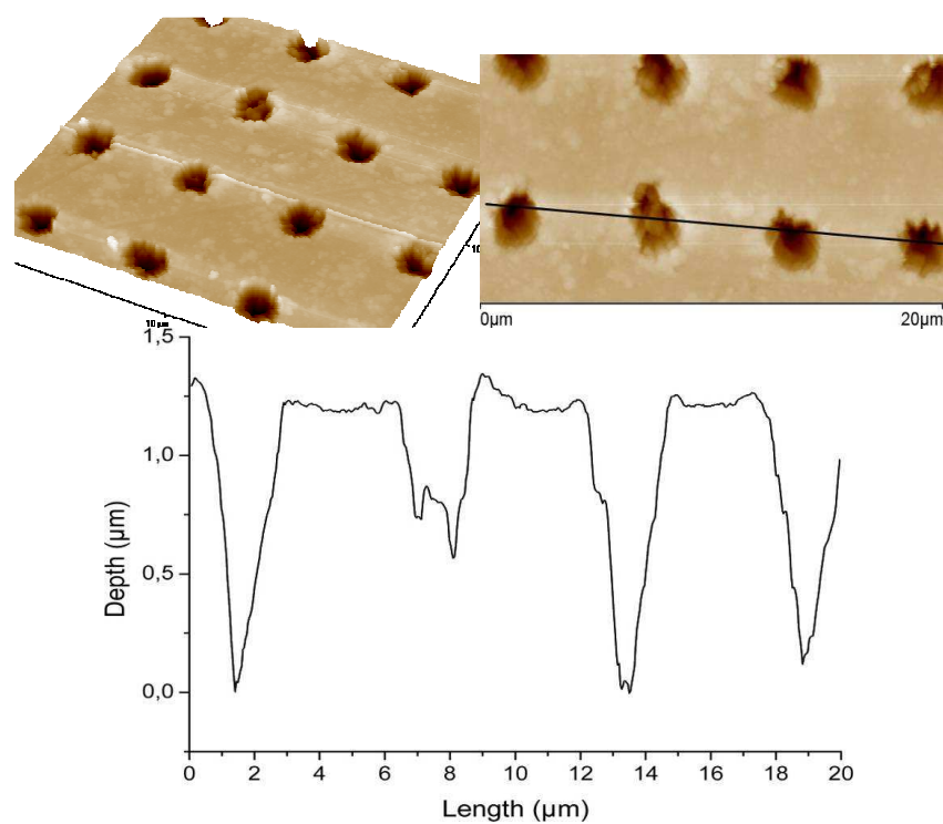
SI-2. AFM image and profile of the master mold B with holes of 1 micron depth.
