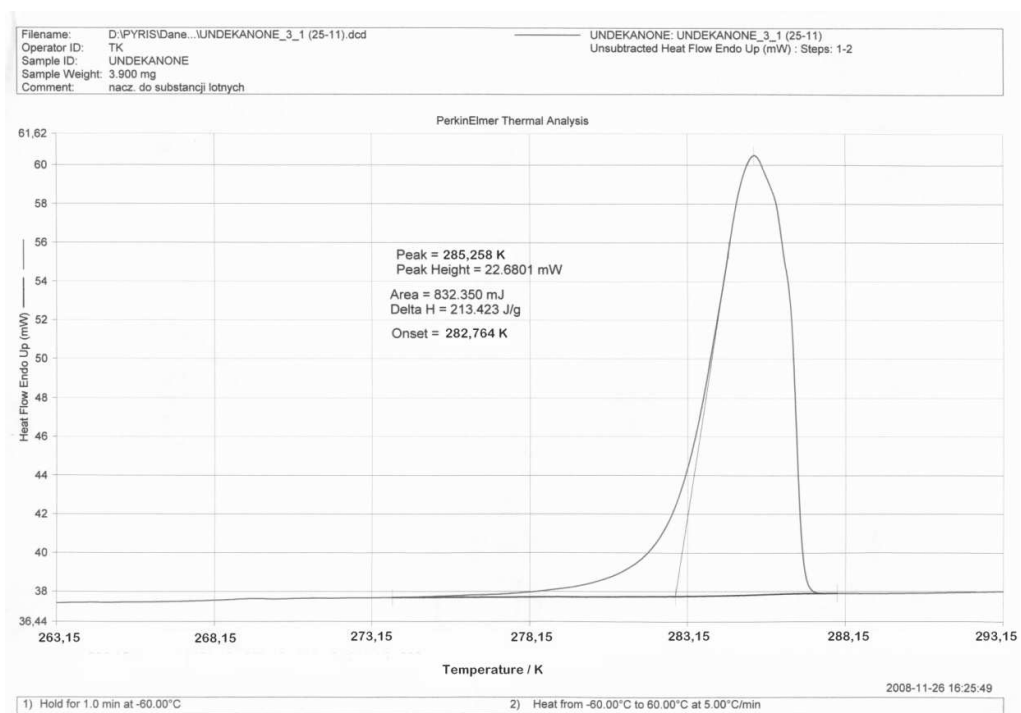
Figure 3S. DSC plot of undecan-2-one.
