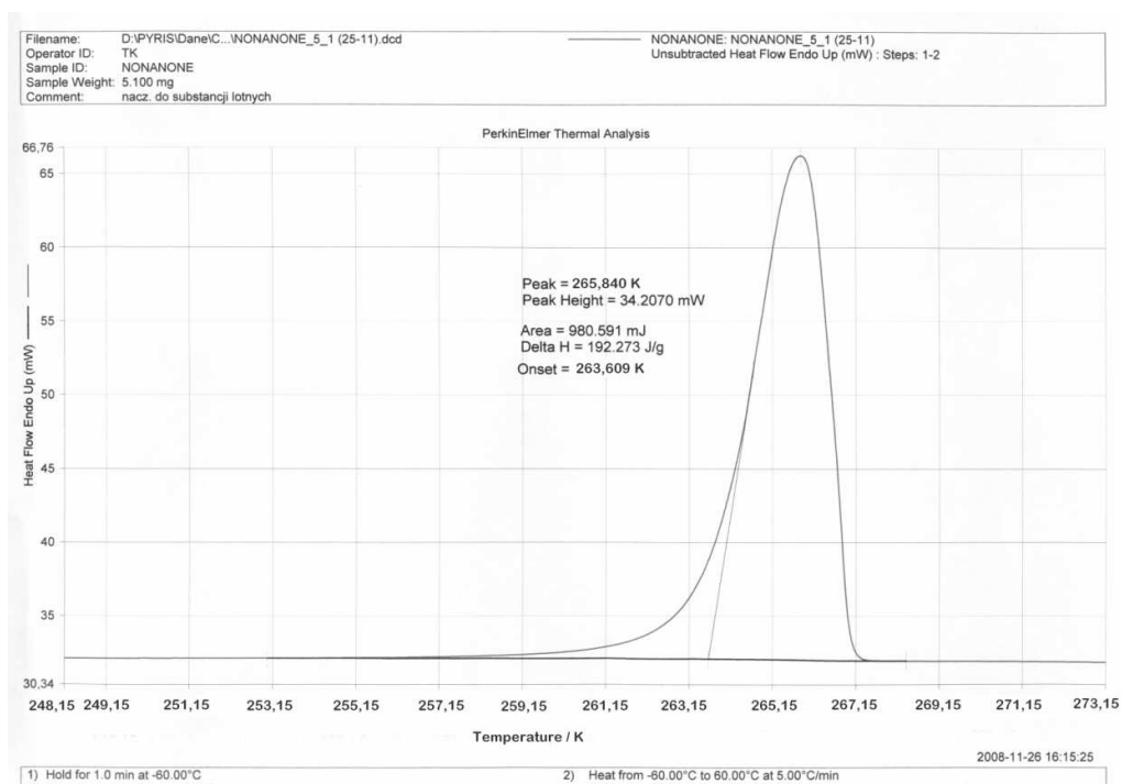
Figure 2S. DSC plot of nonan-2-one.
