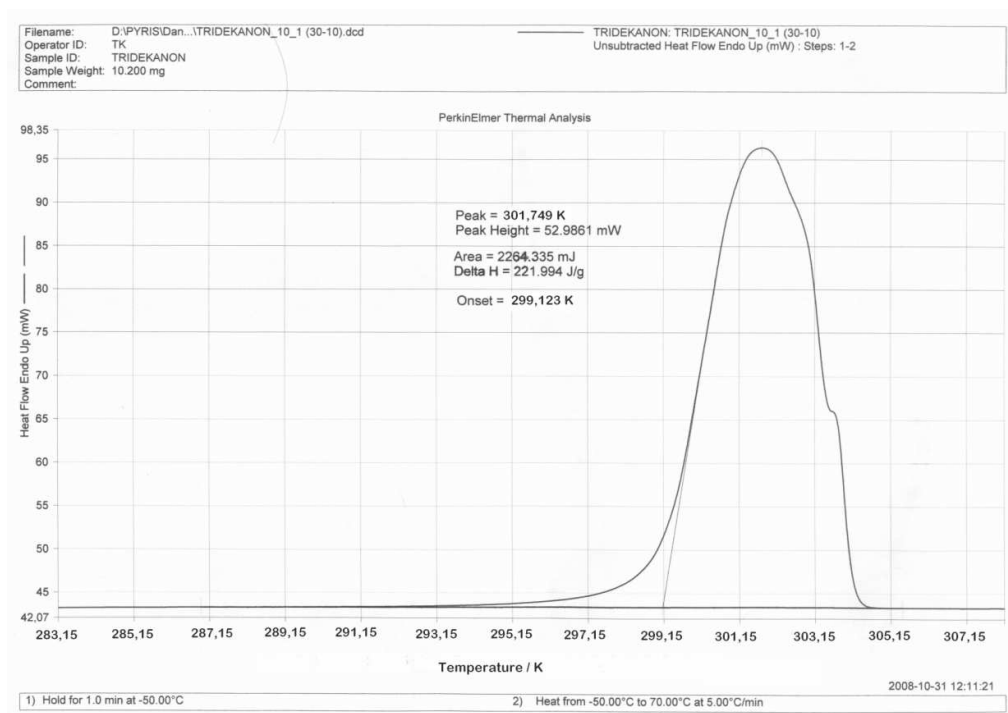
Figure 5S. DSC plot of tridecan-2-one.
