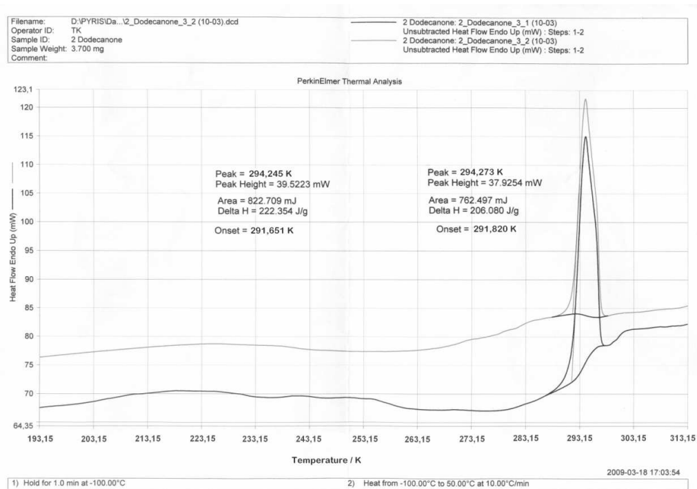
Figure 4S. DSC plot of dodecan-2-one.
