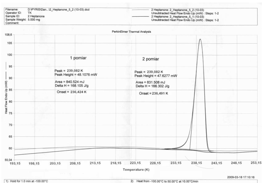
Figure 1S. DSC plot of heptan-2-one.
