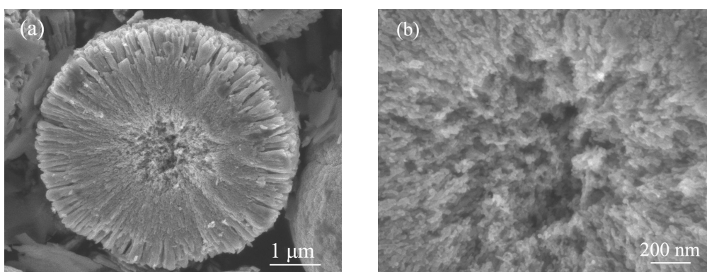
Figure S2 the structure evolution of the sphere from nanoparticles to nanorods: (a) low magnification and (b) high magnified SEM images of a defined sphere
