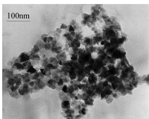
Figure S1 TEM image of products synthesized in glycerol solution
