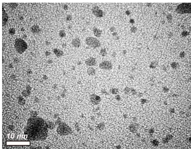
Figure S3 TEM image of the nanostructures prepared by using binary Pd (0.05 mmol)-Pt (0.05 mmol) precursors.
