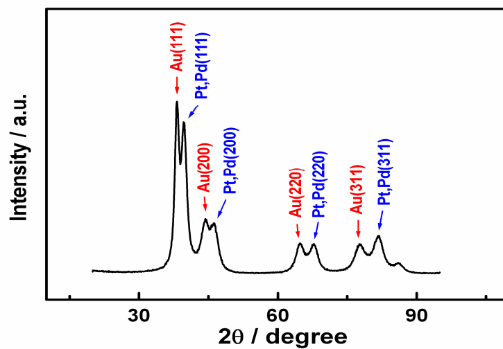
Figure S1 Wide-angle XRD pattern of the Au@Pd@Pt triple-layered core-shell structured nanoparticles.
