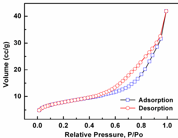
Figure S2 N 2 adsorption-desorption isotherm of the Au@Pd@Pt triple-layered core-shell structured nanoparticles.
