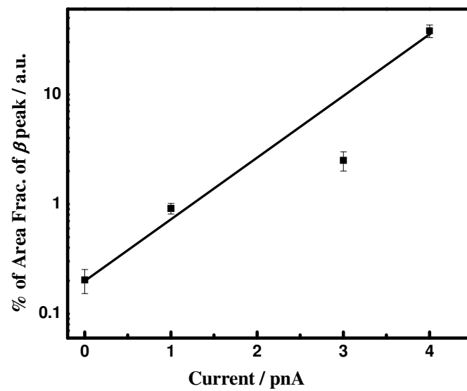
Figure S1: Percentage of area fraction of \beta peak as a function of beam current evaluated from the respective peak area given in figure 1 (b).
