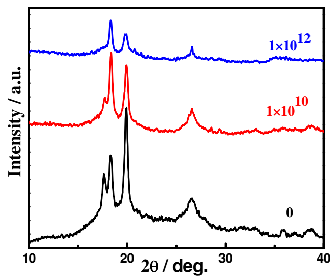
Figure S2: XRD patterns of pure PVDF and irradiated PVDF at different fluences having 0.5 pA beam current. The number “0” indicates the zero fluence.
