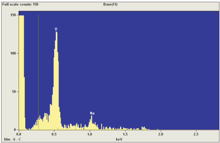
Glass surface after oxygen plasma (2kV)
