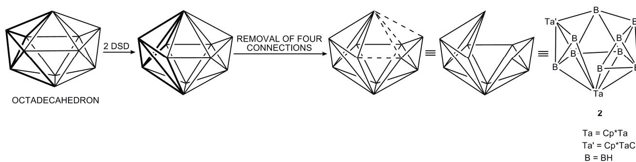
Figure S1. The observed geometry of 2 is generated from an octadecahedron by performing two dsd rearrangements (bold lines) followed by removal of four connections (dashed lines).
