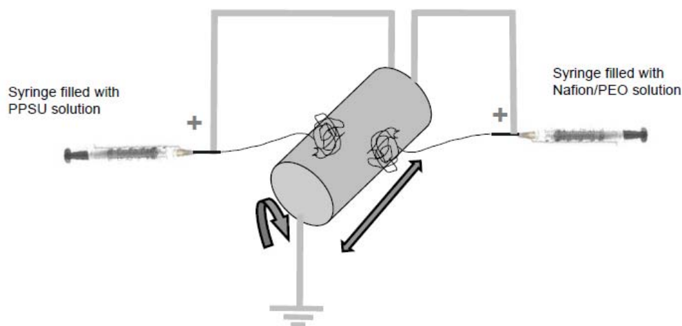
Figure S1. Schematic of dual-fiber electrospinning experiment. The collecting drum rotates and oscillates horizontally for random orientation and uniform distribution of the nanofibers.
