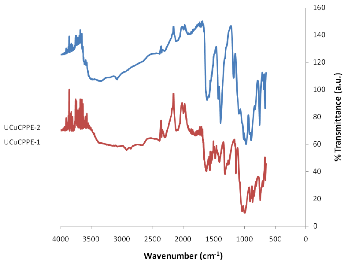
Infrared spectra of UCuCPPE-1 and UCuCPPE-2
