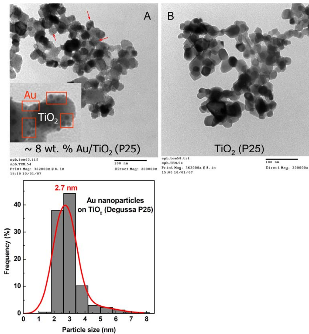
Figure SI 1. Transmission electron microscopy (TEM) images of (A) the 8 % w/w Au/TiO 2 sample and (B) the Degussa P25 TiO 2 sample; (C) Au particles size distribution of as prepared Au/TiO 2 sample made from measurement of 80 particles diameters.
