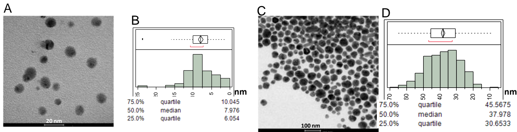
Supporting Information Figure S3: Shape and size distribution of silver nanoparticles: A-B) PVP 8 ; C-D) PVP 38 ; Sample images were obtained from transmission electron microscopy, and size distributions are based on the TEM pictures.
