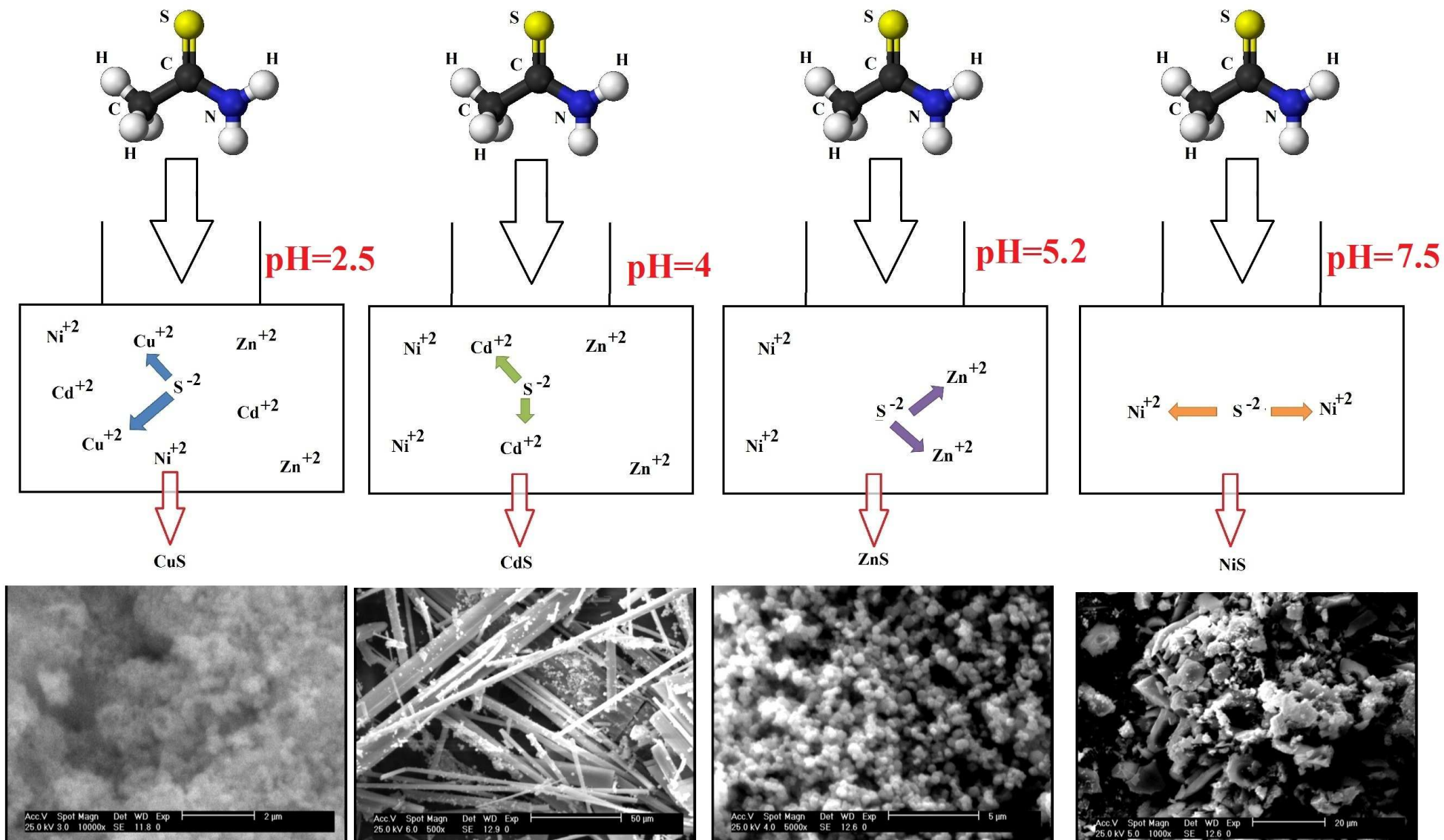
Selective metal precipitation at various pH
