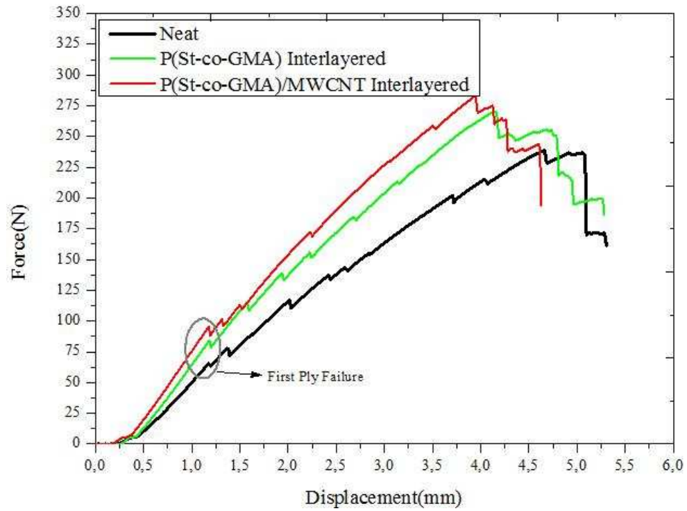
Figure S1. Representative force-displacement test curves for [90/0/90] orientation nanofiber reinforced prepreg laminates (43,44)
