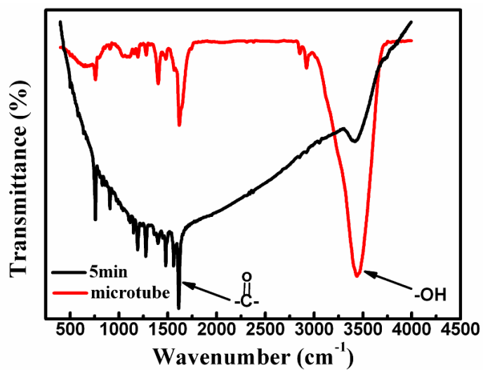
Figure S2 IR spectra of the samples collected at the ripening time of 5 min and 8 h.
