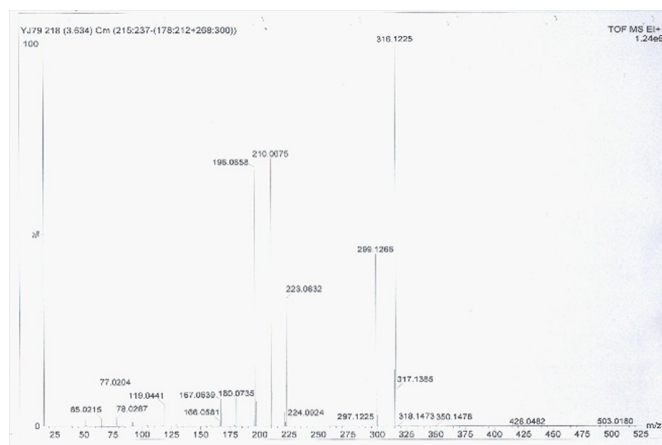
Figure S1. MS of the as-synthesized salophen
