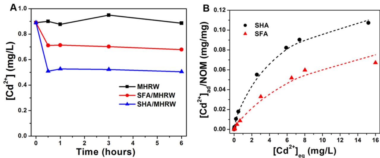
Figure S5. Cd 2+ adsorption on NOM. (A) Time dependent measurements of Cd 2+ concentration in MHRW and NOM, showing rapid Cd 2+ adsorption on NOM. The experiment was conducted at 25 °C and NOM was added at 20 mg/L. (B) Equilibrium adsorption isotherms for Cd 2+ binding to SHA, SFA at 25 °C. NOM was used at 20 mg/L in MHRW, and the NOM/adsorbed-Cd 2+ phase was removed by centrifugal ultrafiltration prior to ICP analysis. The dashed lines give the calculated adsorption isotherms derived from Langmuir-Freundlich isotherm model, where Q_{\max} (SHA) = 0.156 mg/mg, K_{SM} (SHA) = 0.249 L/mg, n (SHA) = 0.830, and Q_{\max} (SFA) = 0.131 mg/mg, K_{SM} (SFA) = 0.114 L/mg, n (SFA) = 0.890.
