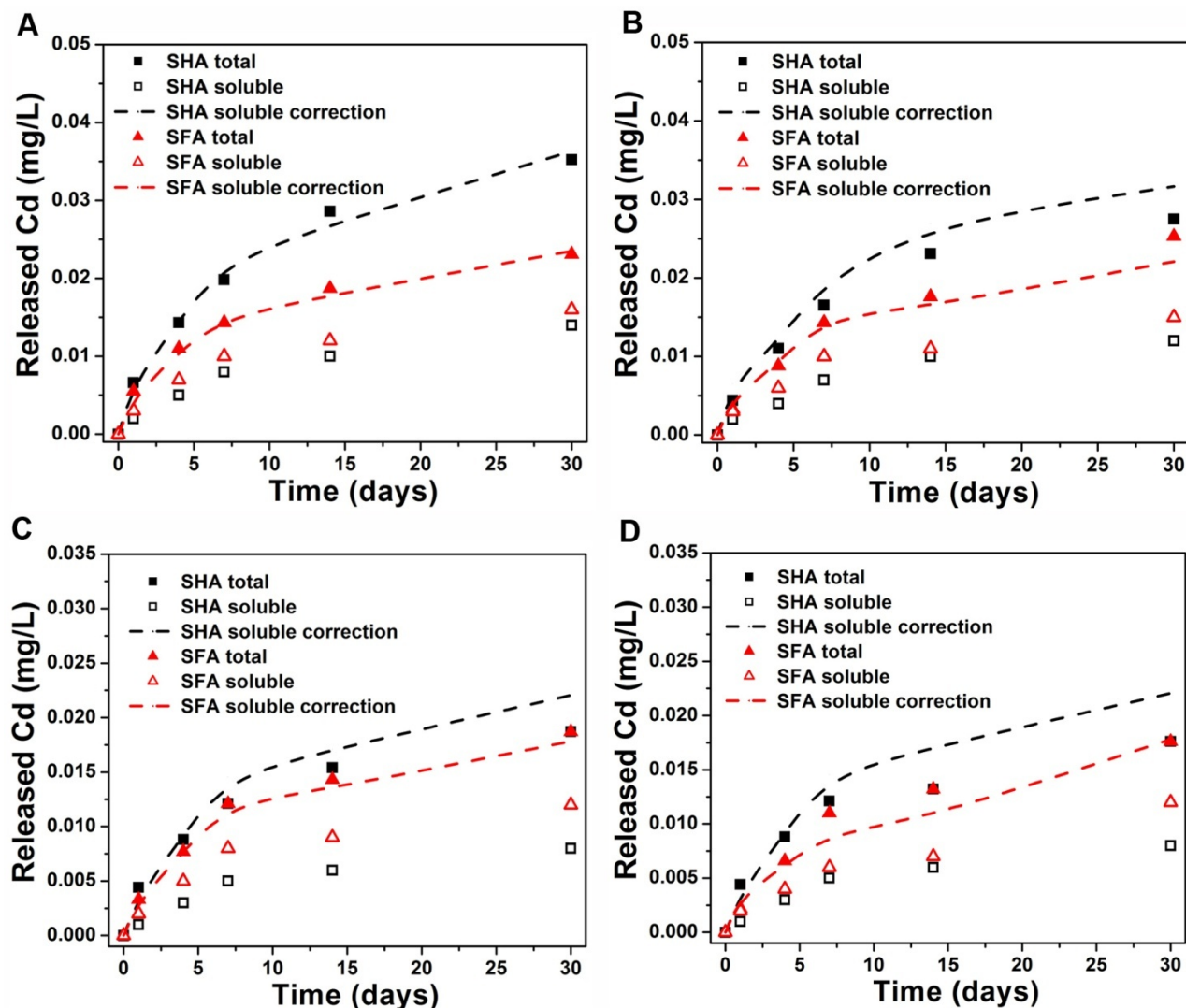
Figure S7. Total and soluble Cd release from QD optic samples in the presence of SHA and SFA (points) and correction of the soluble release for \text{Cd}^{2+} adsorbed on NOM (dashed lines). (A) Glass protected optic assembly under dark exposure; (B) Glass protected optic assembly under light exposure; (C) QD-embedded polymer under dark exposure; and (D) QD-embedded polymer under light exposure. The dashed lines give the calculated total Cd release based on Langmuir-Freundlich fitting of soluble Cd, suggesting the difference between total and soluble Cd is primarily due to ion adsorption on NOM.
