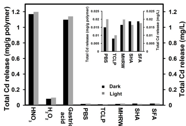
Figure S2. Total Cd release after 30 day dark or light exposure to simulant fluids. QD-embedded polymers were exposed at 1 mg polymer/mL solution, and were rotated under dark or ambient light at 60 rpm.
