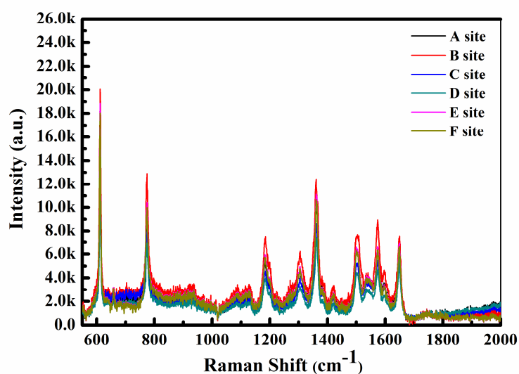
Figure S1. SERS spectra collected from the randomly selected six sites of the Ag-capped SiNW arrays after the replacement reaction with 0.04 mM H AuCl 4 aqueous solution. The reaction temperature is 60 °C.
