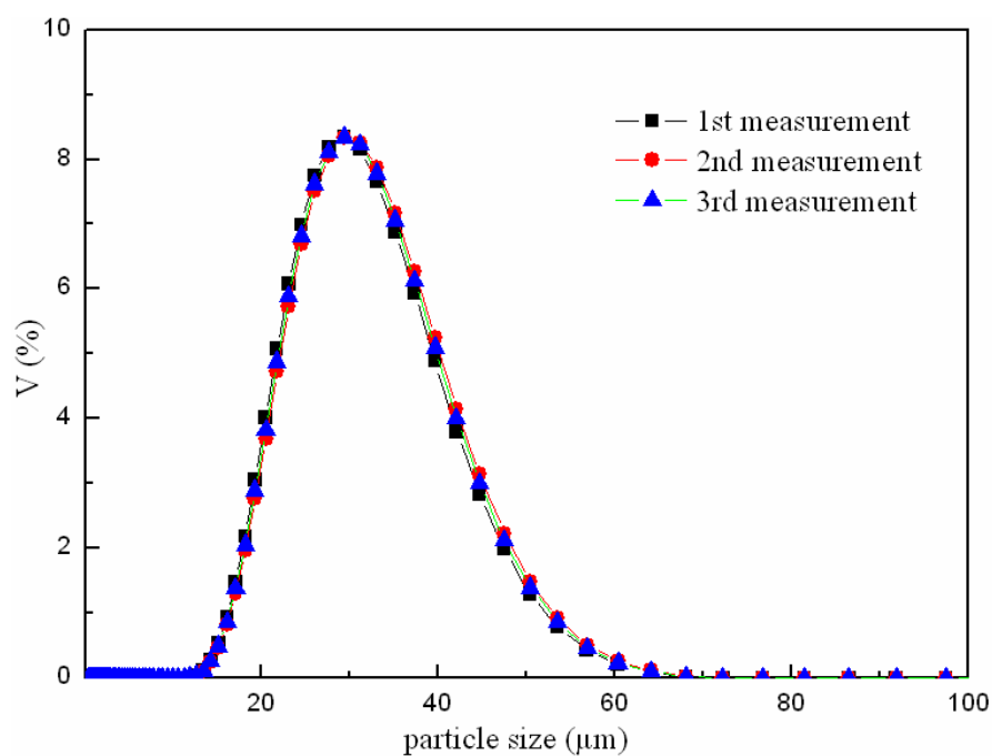
Fig S1. Three measurements of PSDs of produced crystals.
