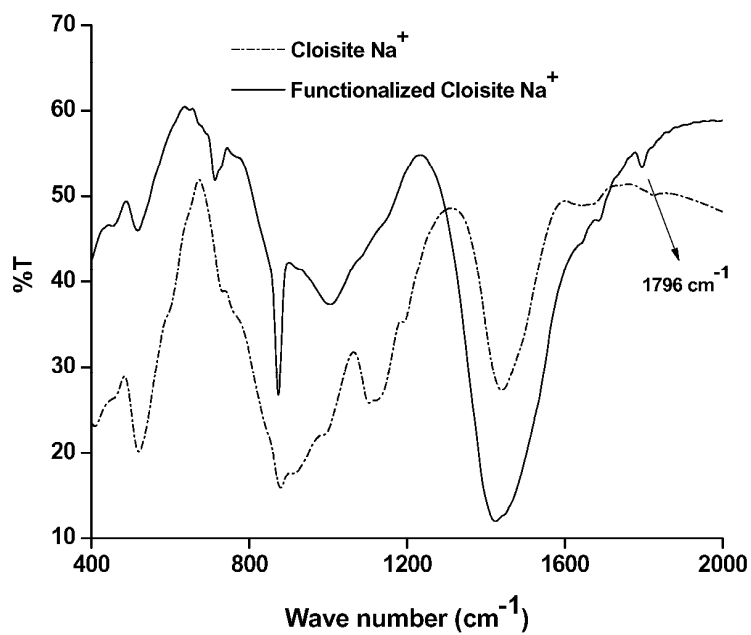
Figure S1: FT-IR spectra of Cloisite Na + and functionalized Cloisite Na +
