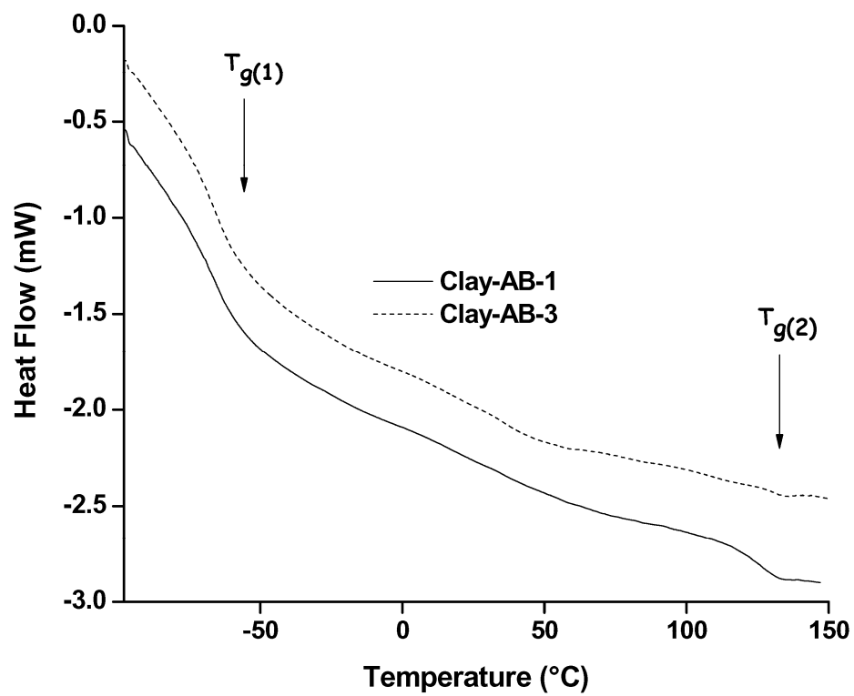
Figure S3: DSC traces of block copolymer/clay nanocomposites
