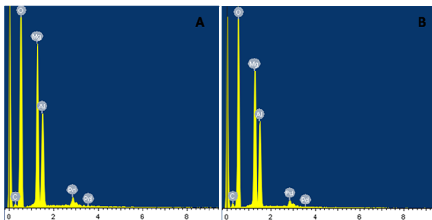
Figure S1 EDX spectra of SWPL catalyst (A) and CPL catalyst (B)
