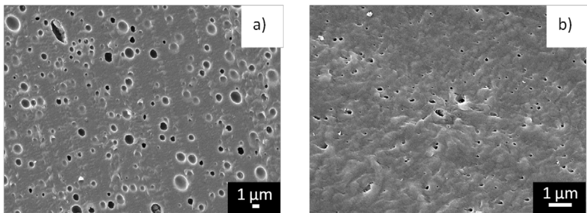
Figure 11. SEM micrographs of 92/8 vol% cocontinuous blends after PEO extraction: a) PE/PEO, b) PE-g-MA/PEO.
