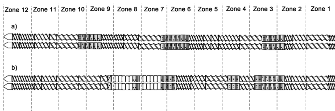
Figure 10. a) Low shear screw configuration, b) high shear configuration.
