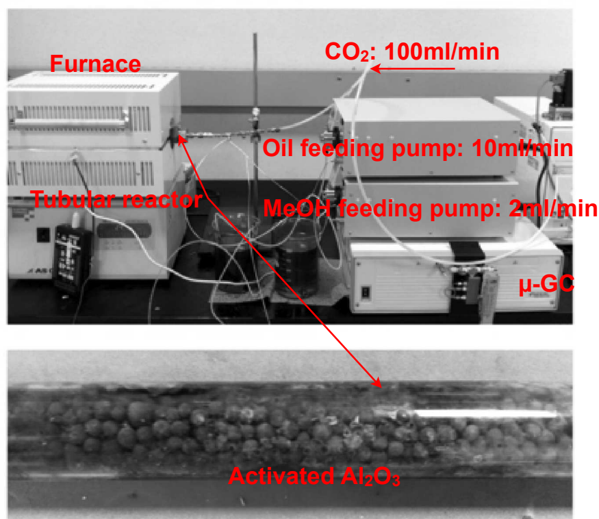
Figure SI-1. Overall illustration of experimental setup and inside of reactor
