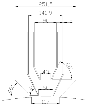
Figure 2 Size parameters of primary nozzle
