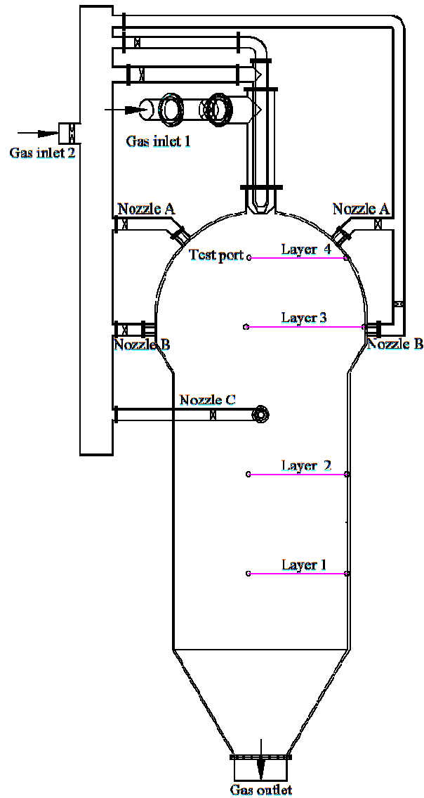
Figure 3. Schematic of the 500t/d pressurized entrained-flow gasifier by two-stage oxygen.
