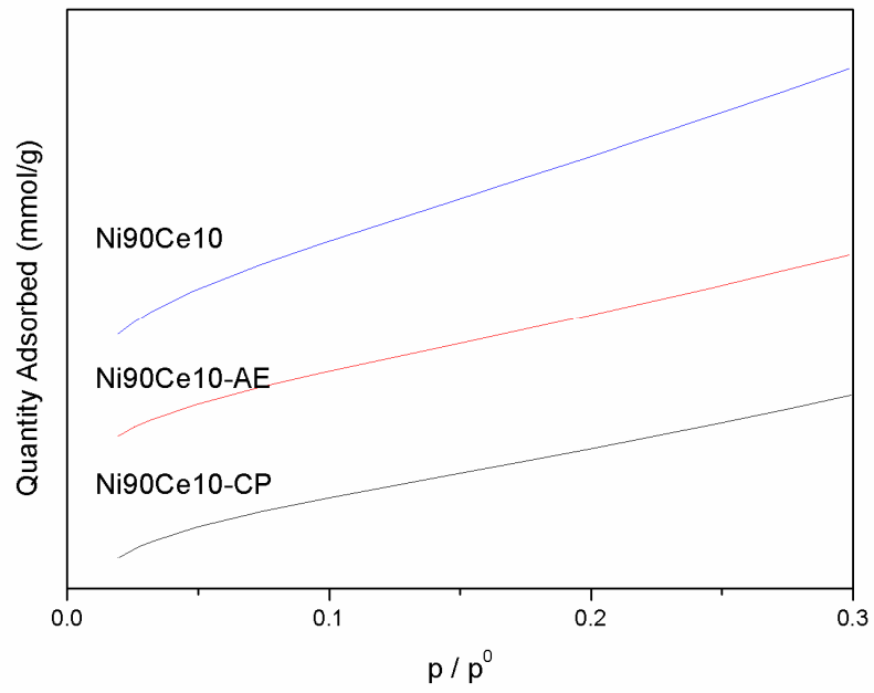
Figure S2. N 2 adsorption isotherms of NiCe mixed oxides catalysts prepared by different methods.
