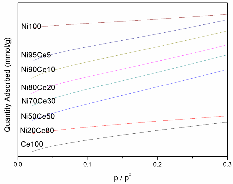
Figure S1. N 2 adsorption isotherms of NiCe mixed oxides catalysts with different Ni/Ce ratios.
