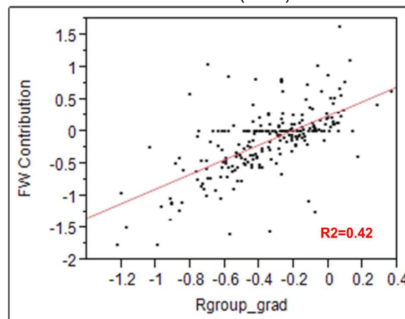
IL4 dataset (n=241, outliers=11)
