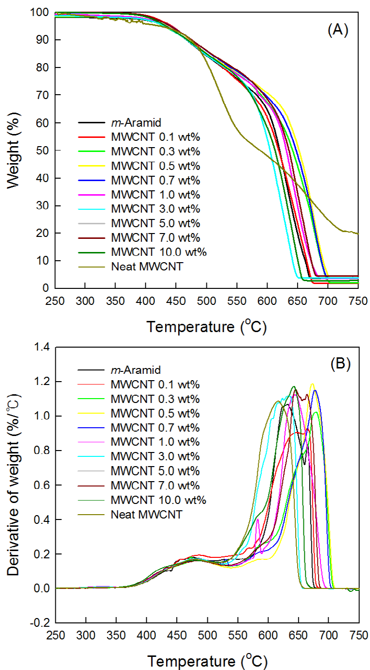
Figure S1. TGA thermograms of the neat m -aramid and its composite films with different MWCNT contents under the air condition at a heating rate of 10 °C/min.
