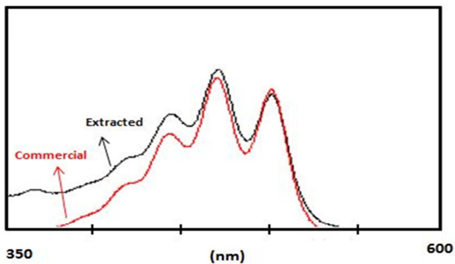
Fig.1A- UV-Vis spectra of lycopene extracted from tomato and commercially available lycopene.
