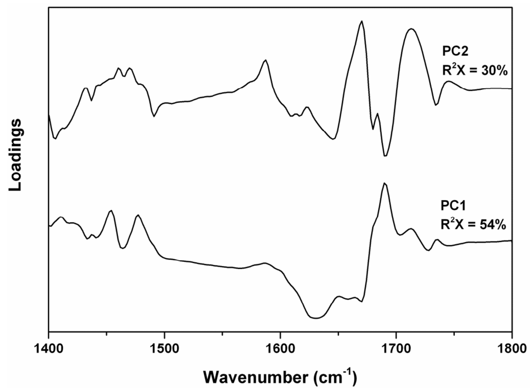
Figure 3. Corresponding PCA loadings plot of the scores plot obtained at pH 6.8
