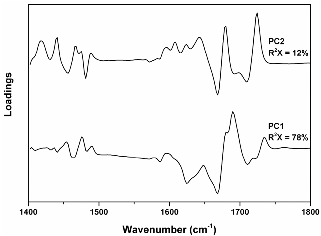
Figure 2. Corresponding PCA loadings plot of the scores plot obtained at pH 4.5
