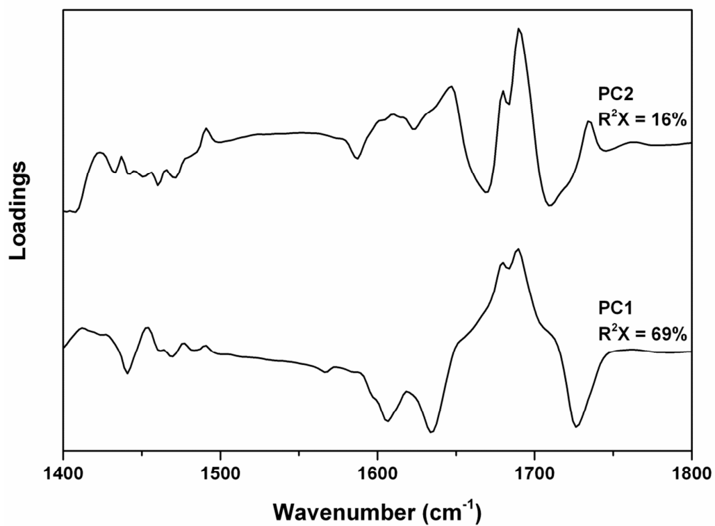
Figure 1. Corresponding PCA loadings plot of the scores plot obtained at pH 1.2
