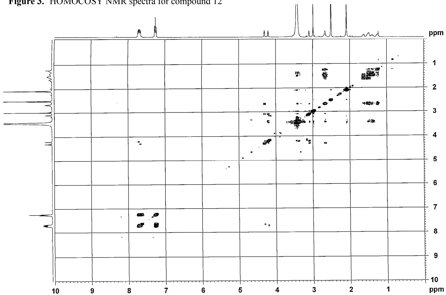
Figure 3. ^1\text{HOMOCOSY} NMR spectra for compound 12
