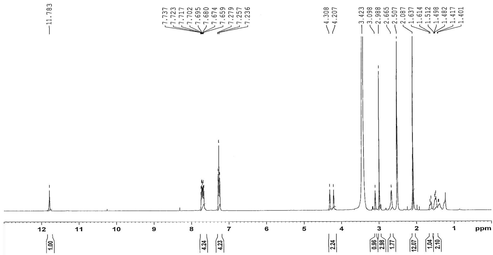
Figure 1. ^1\text{H} NMR spectra for compound 12
