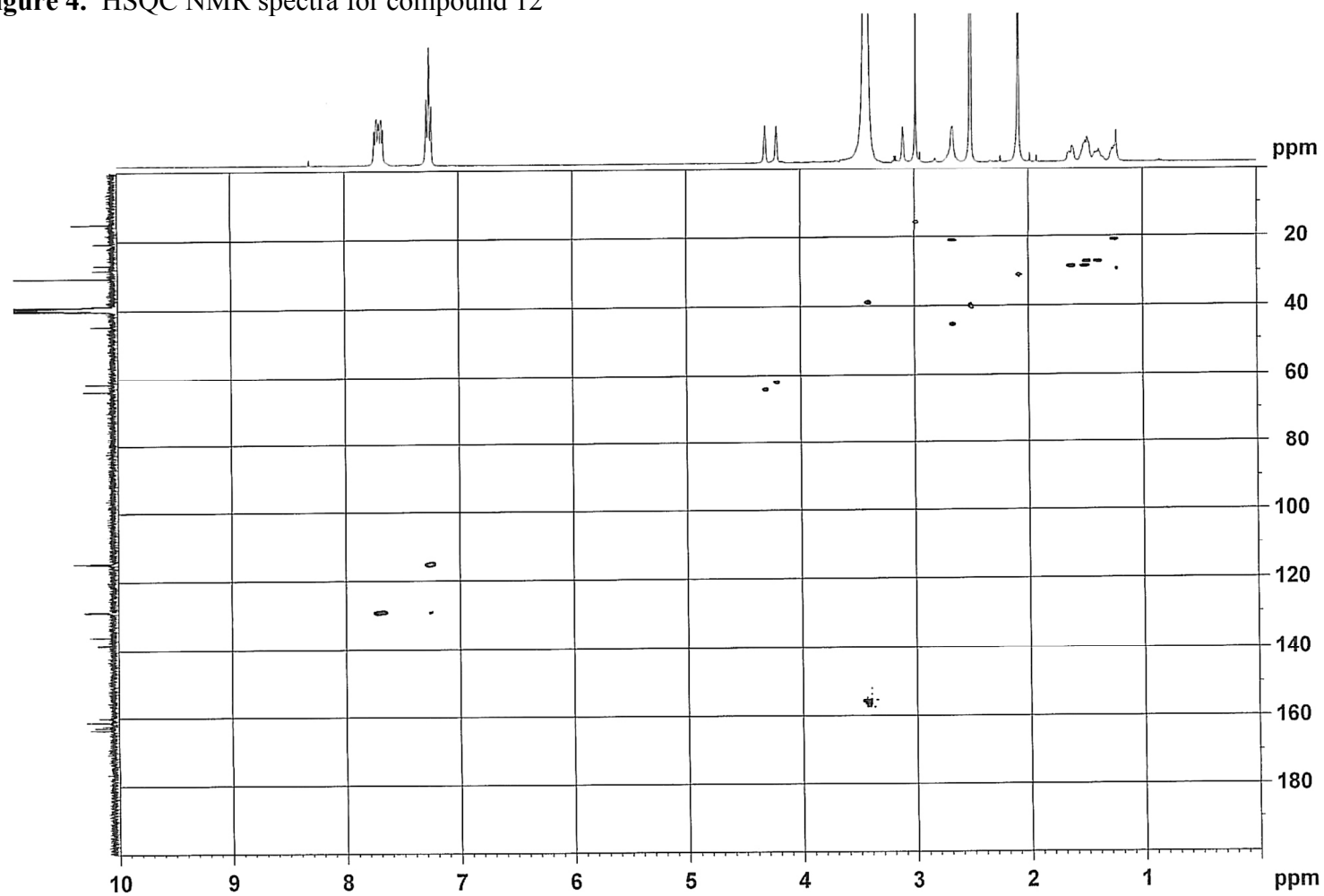
Figure 4. HSQC NMR spectra for compound 12
