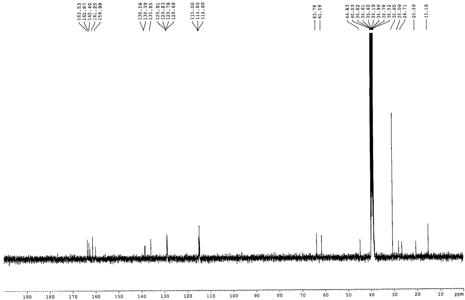
Figure 2. ^{13}\text{C} NMR spectra for compound 12
