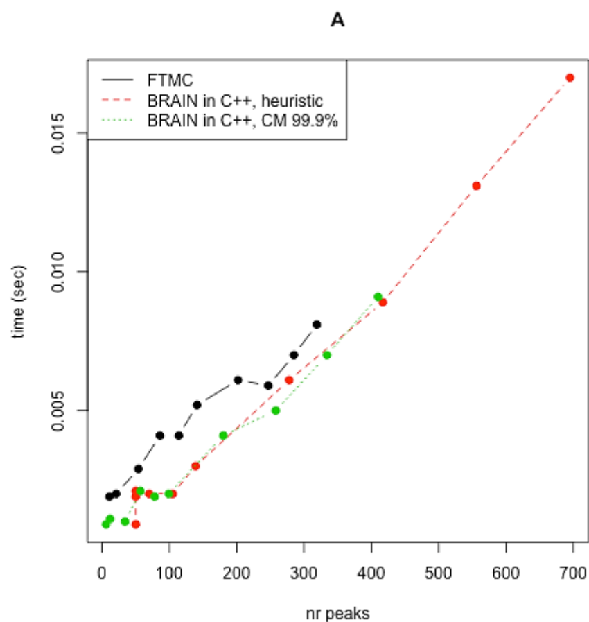
Figure S1: Average system time elapsed in function of the number of computed peaks for FTMC and BRAIN in C++ with input file containing 100 times the same molecules for each averagine molecule (shown system times are divided by 100). The data points corresponding to the same number of peaks do not correspond to the same molecule.
