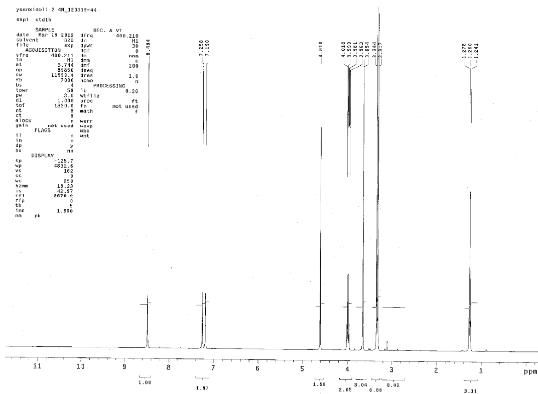
^1\text{H} NMR spectra for [Emim][DMP]
