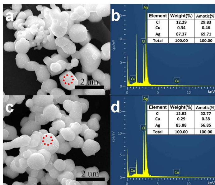
Figure S1. (a) FESEM image of as-prepared Cu(II)/AgCl (0.05M) and (b) its corresponding EDX; (c) FESEM image of 5-time repeated Cu(II)/AgCl (0.05M) and (d) its corresponding EDX.
