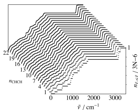
a) MFDs of all cis -Polyenes from C_4 to C_{50} B3LYP/6-31G(d)
