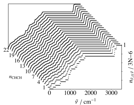
a) MFDs of all cis -Polyenes from C_4 to C_{50} B3LYP/6-311G(d,p)
