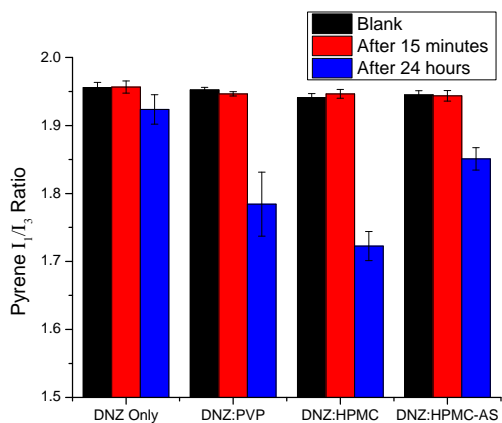
Supplemental Figure 1. Pyrene emission fluorescence ratios for solutions containing crystalline danazol.
