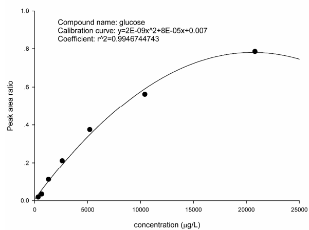
Figure S2. Calibration curves of glucose (quadratic fits)
