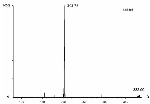
Figure S1. Daughter scan of m/z 383, glucose, electrospray in positive ion mode (collision energy 20 V) with daughter ion at m/z 203.
