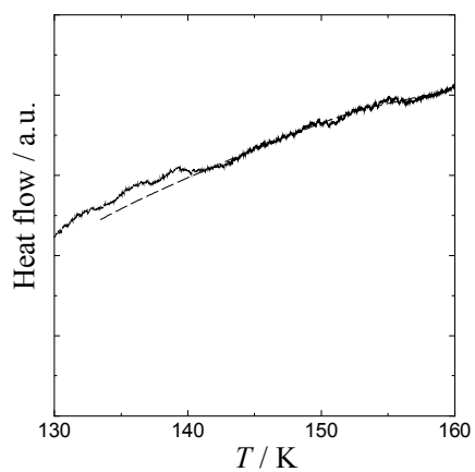
Figure. S1 Heat-flow curve, scanned at a heating rate of +3 K/min, for the ACIBA crystal: A dashed line is a guide for eyes.
