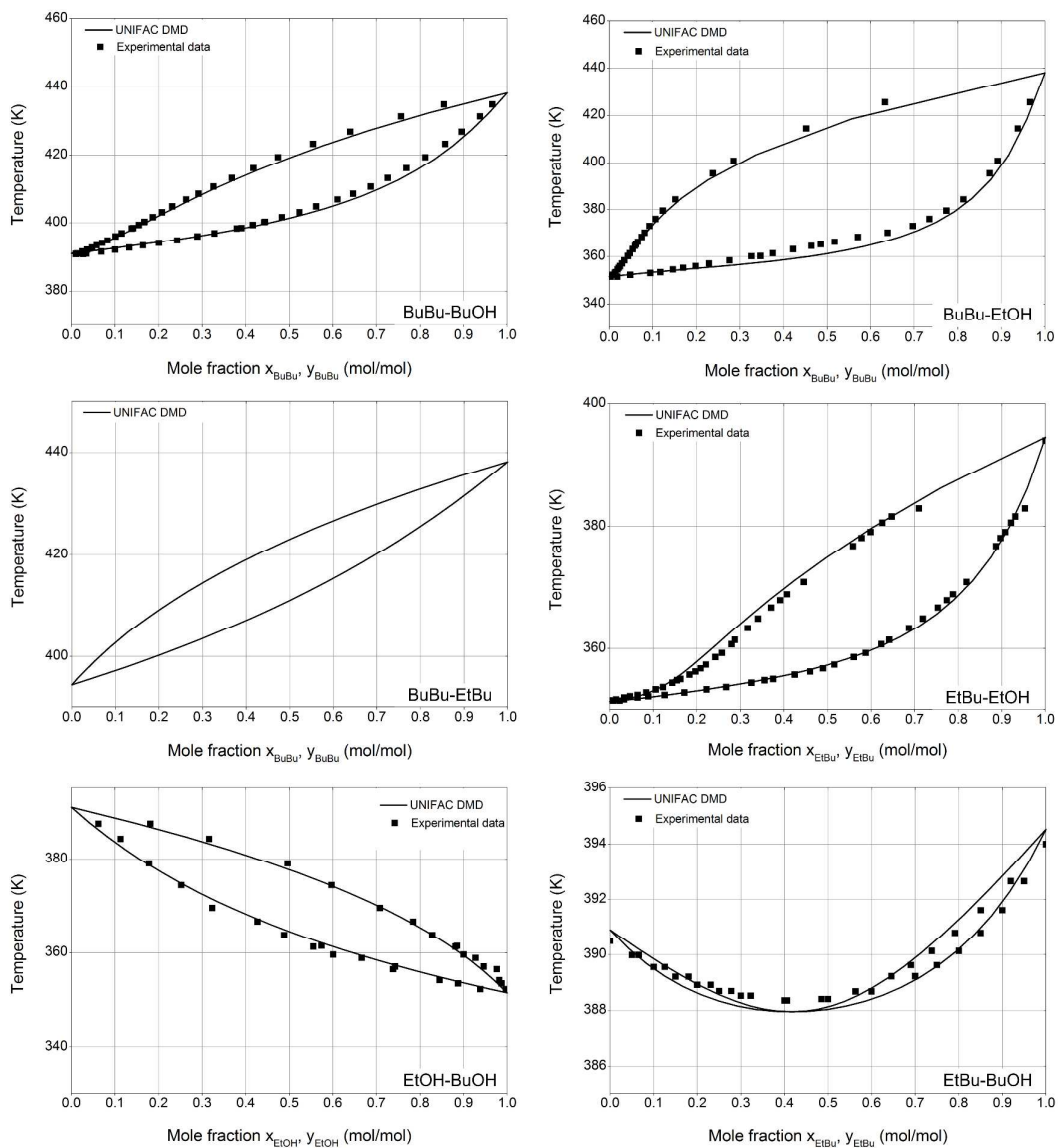
Figure S2. VLEs of all main components calculated with UNIFAC DMD and compared to available experimental data from literature
