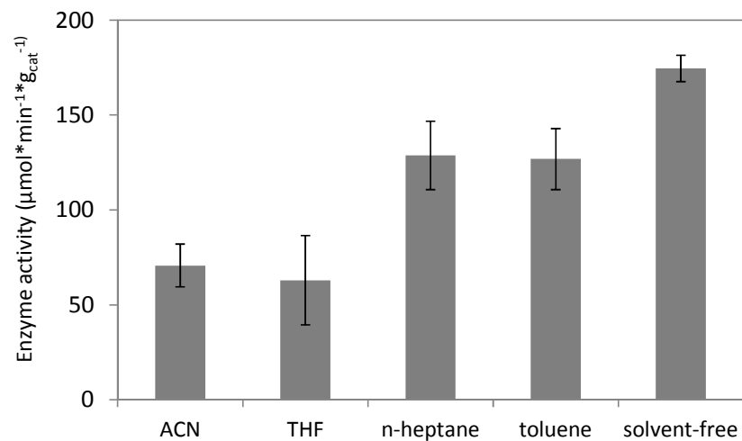
Figure S1 - Solvent screening for enzyme activity tests: Lipase CALB activity for transesterification of ethyl butyrate with n -butanol in different solvents and in a solvent-free system. ACN - acetonitrile, THF - Tetrahydrofuran
