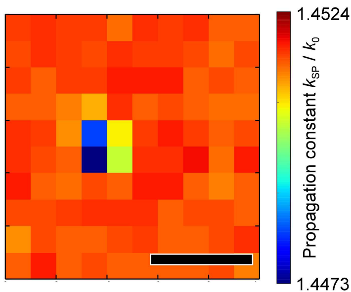
Figure S1. SPR propagation constant of a bare gold film in water measured with SLSPM. The scale bar is 4 \mu\text{m} .
