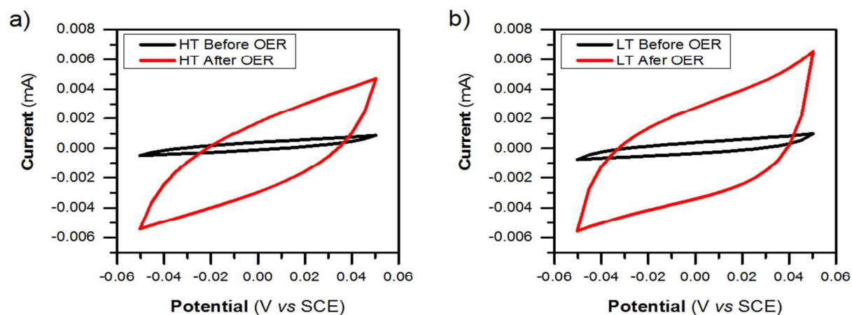
Figure S1: CVs of (a) HT-LiCoO 2 and (b) LT-LiCoO 2 in a non-faradaic region, showing the difference in double layer capacitance before and after OER.
