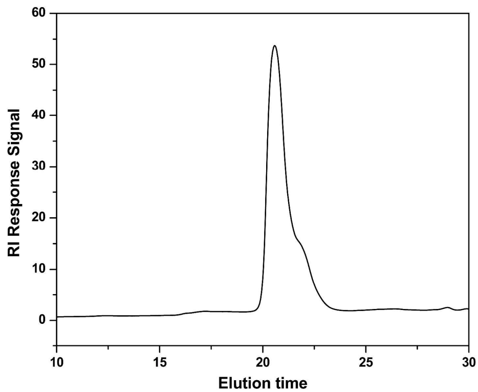
Figure S2. GPC trace of PAE-g-DSMPEG.
