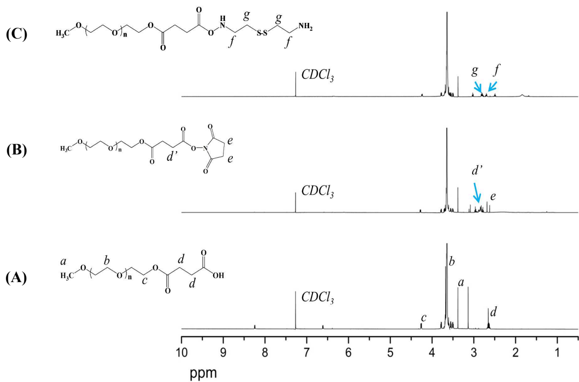
Figure S1. ^1\text{H} -NMR spectra of MPEG-COOH (A), NHS-activated MPEG (B), MPEG-Cystamine (C)
