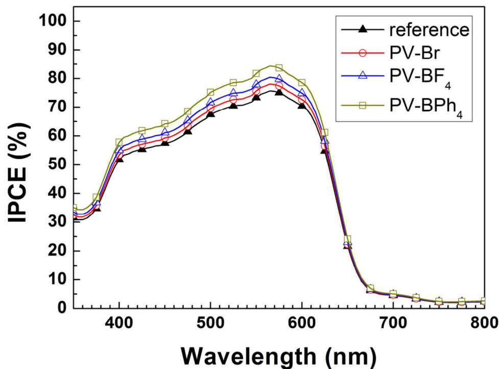
Figure S1. IPCE spectra of the device without PV (filled triangle), with PV-Br (open circle), with PV-BF 4 (open triangle), and with PV-BPh 4 (open square).
