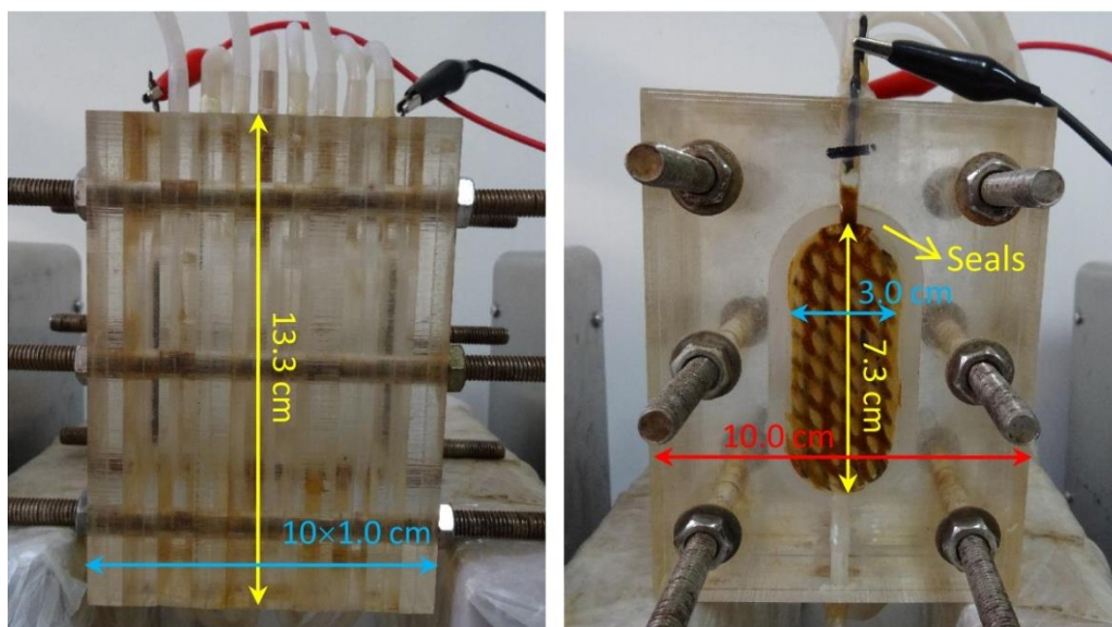
Figure S1. The digital photo of ED setup with geometric characteristics in detail.
